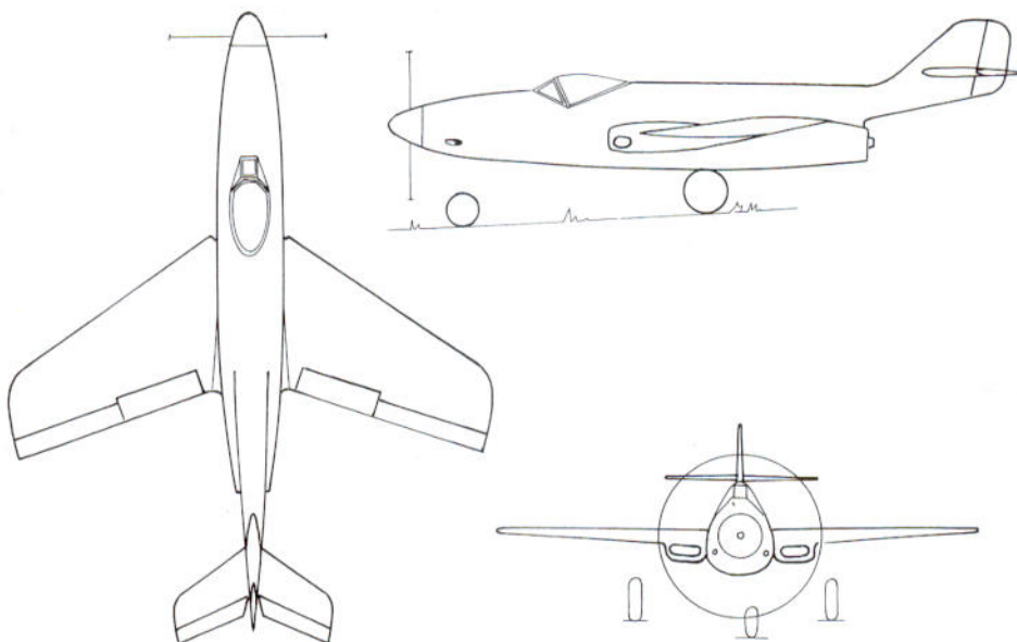
Focke-Wulf turboprop strike fighter.
