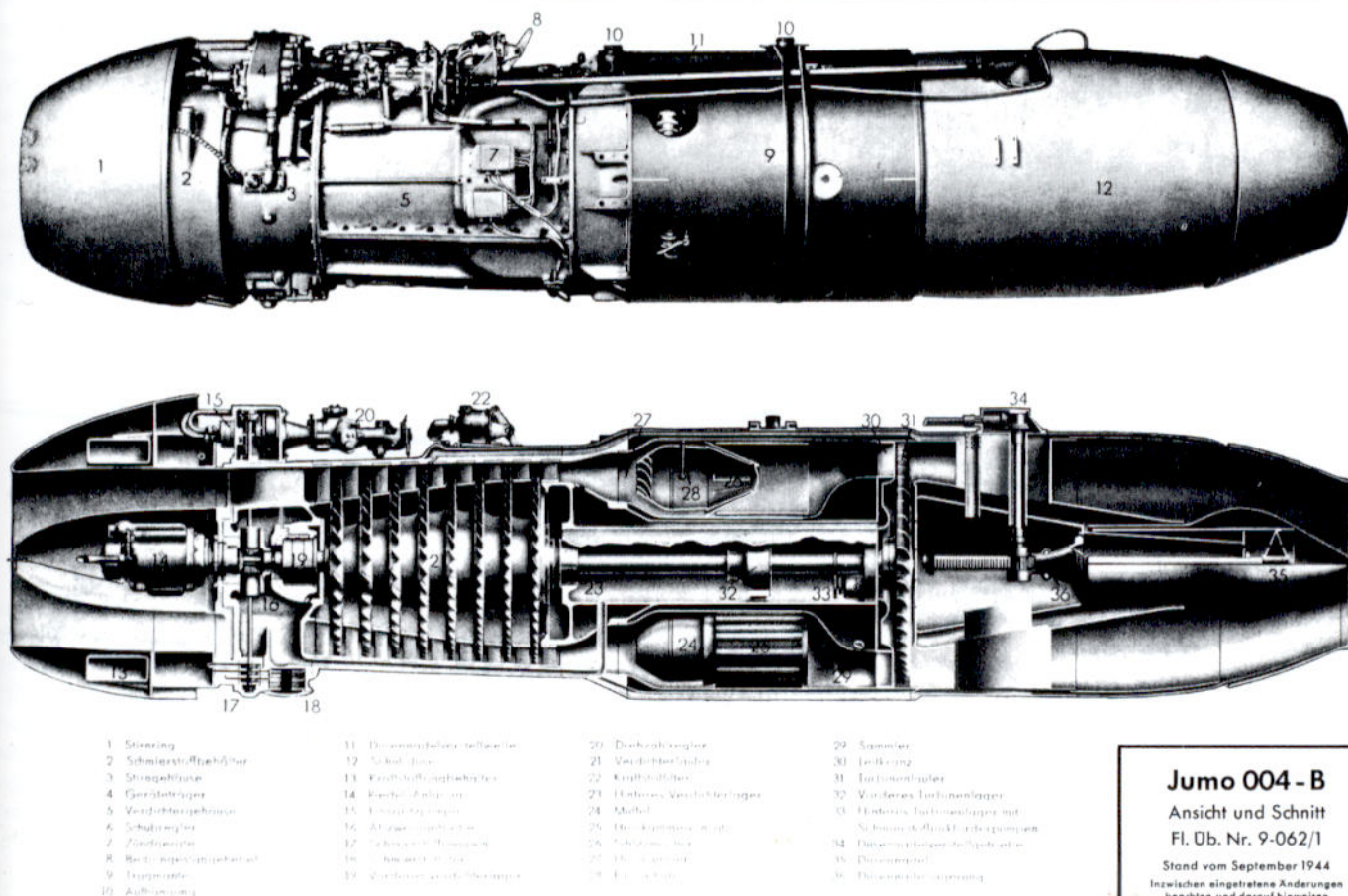
The Junkers Jumo 004 turbojet used throughout the P.1092 project; illustrated is the series production 004B variant.
