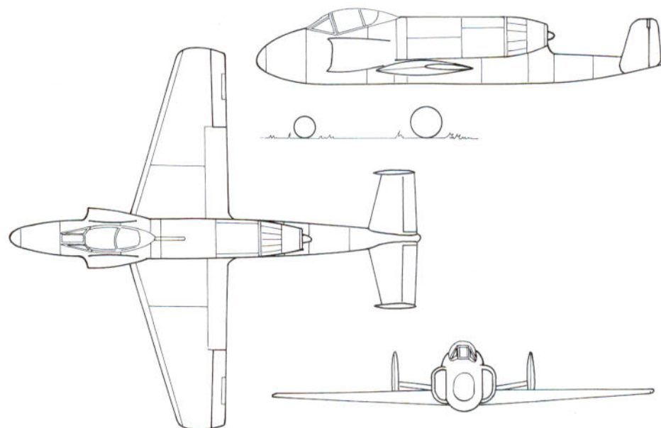
Third Focke-Wulf design for the air superiority fighter.
