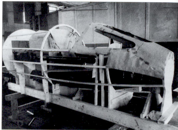
P.1112 forward fuselage mock-up at Oberammergau, April 1945.
