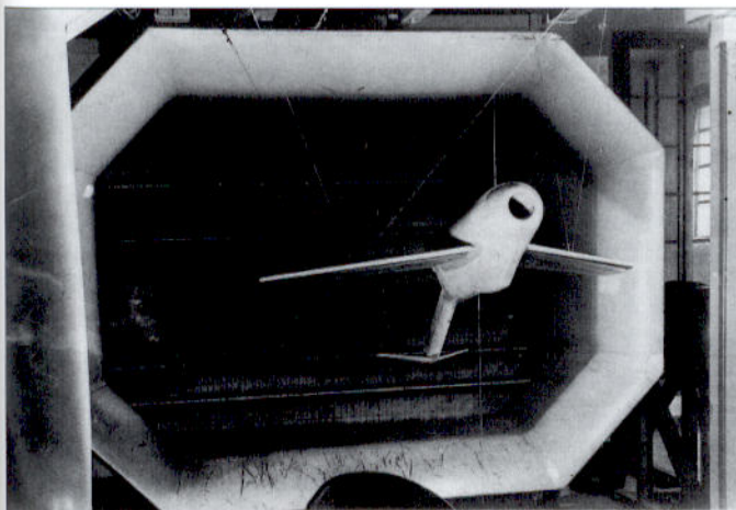
Full model of the Ta183 inverted in the wind tunnel at the end of 1944.
