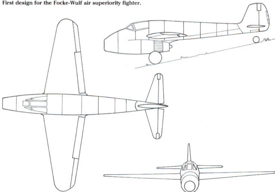
First design for the Focke-Wulf air superiority fighter.
