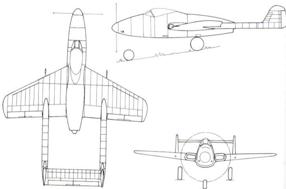
Focke-Wulf's turboprop strike fighter; the seventh design.
