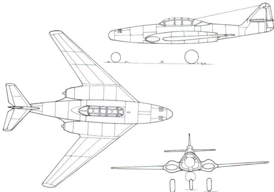
Messerschmitt Me 262 night fighter with HeS 011 turbojets
