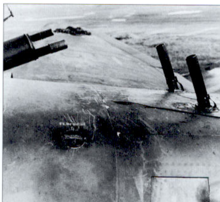
Two MK 1088 30mm cannon protruding from the fuselage of a Junkers Ju88G-6 – the upward-firing Schräge Musik anti-bomber weapon.
