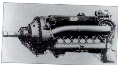
Daimler-Benz DB 628 high altitude engine.
