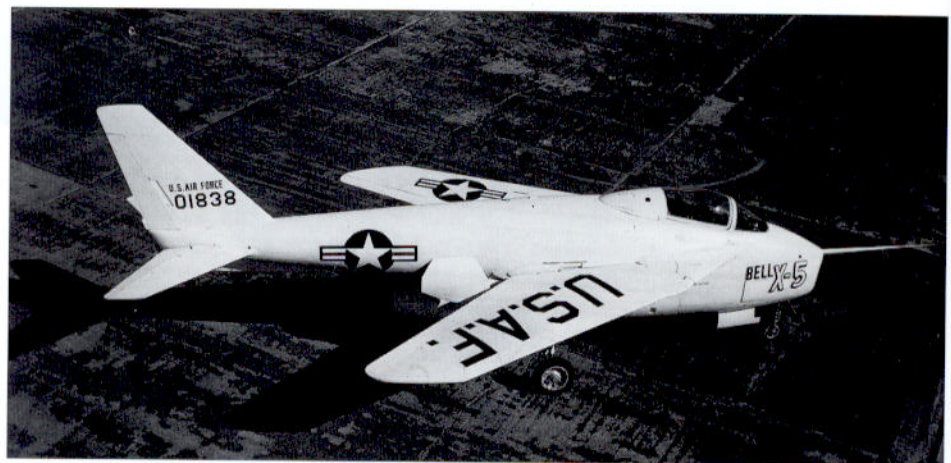
The world's first variable geometry aircraft, the Bell X-5, which relied heavily on the company's experience of the Messerschmitt P.1101.
