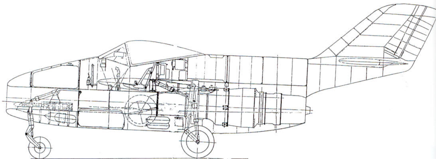
Single jet fighter with HeS 011, Design III, of February 1945.
