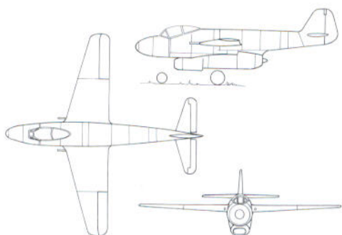
The second Focke-Wulf proposal, with underslung turbojet; initial layout.
