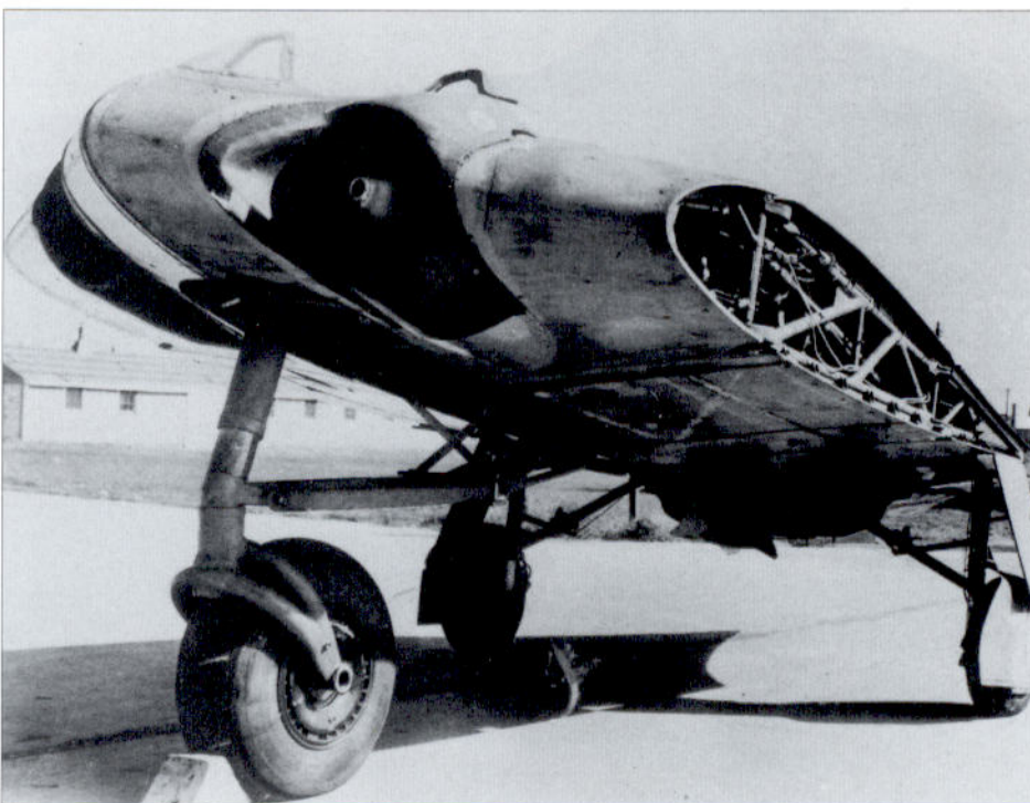
Centre right and bottom right: Two views of the uncompleted HoIX V3 centre section. This is held in storage at Silver Hill, Maryland, by the US National Air and Space Museum.
