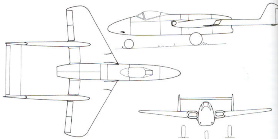
Focke-Wulf Flitzer single jet fighter.
