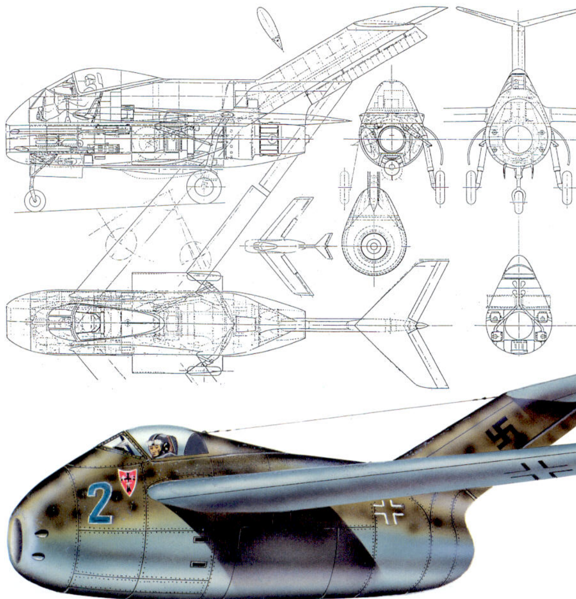
Ta 183 production model powered by the HeS 011 engine (1945).
