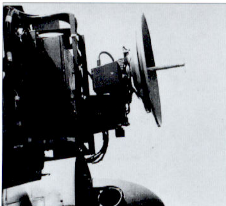
Dish antenna of the FuG 240 'Berlin' radar, predecessor of the FuG 244 'Bremen 0' model.
