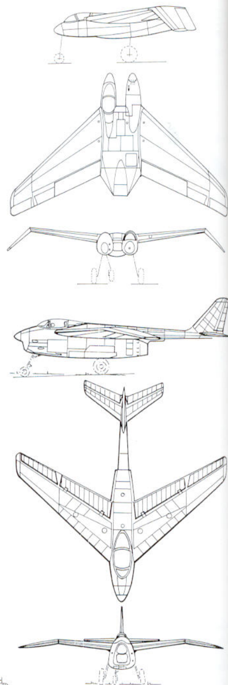
Left and right: Unusual layout of the Heinkel P.1078B project. The use of two 'pods' – one for the pilot and one for the nosewheel and cannon – allowed for a remarkably 'flat' design.
