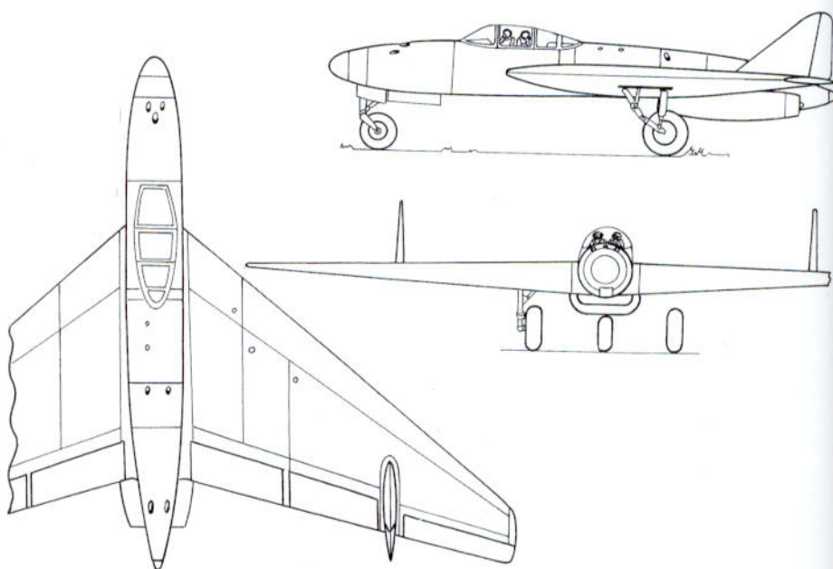
Later version of the Arado Project I (E.583).
