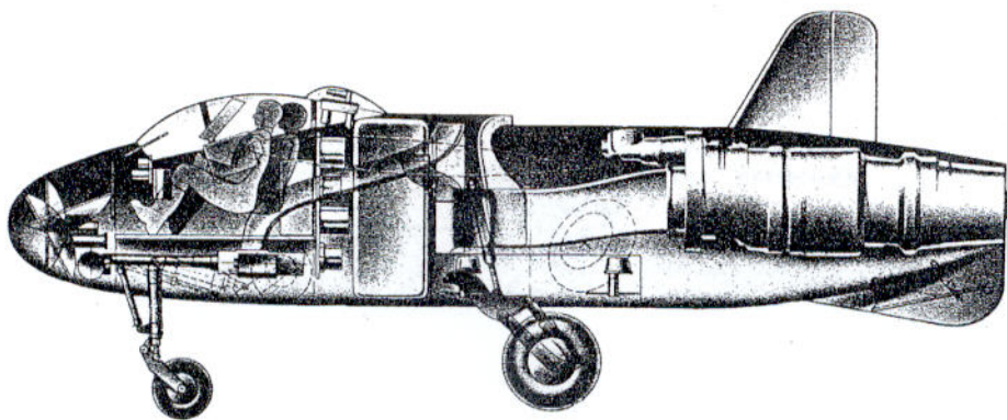
Junkers EF.128 night fighter
