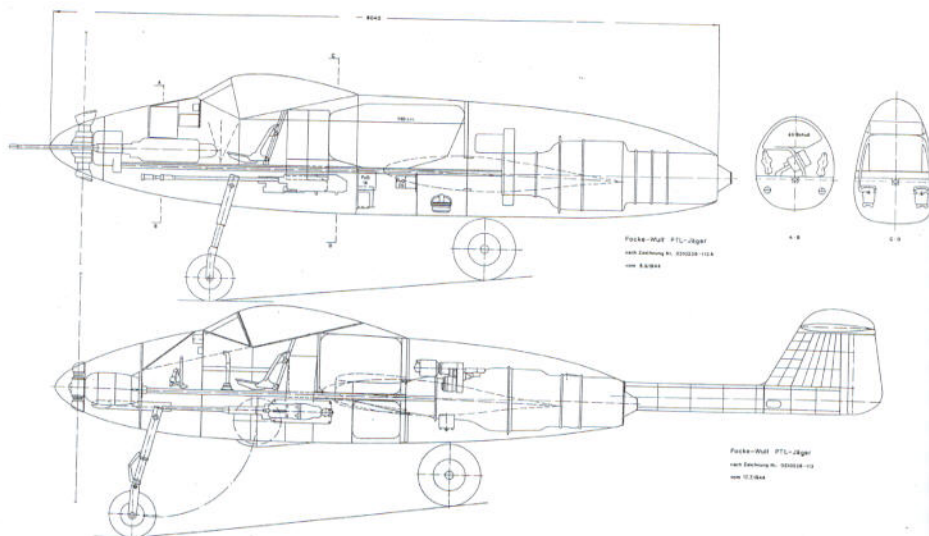
Focke-Wulf's turboprop strike fighter; the seventh design.
