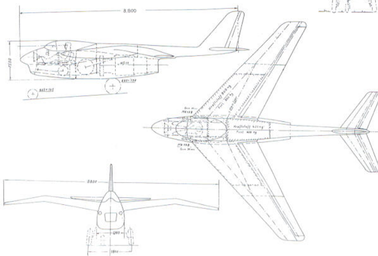
Above, right and below: P.1087A, its exact relationship to the P.1087 study is unconfirmed.
