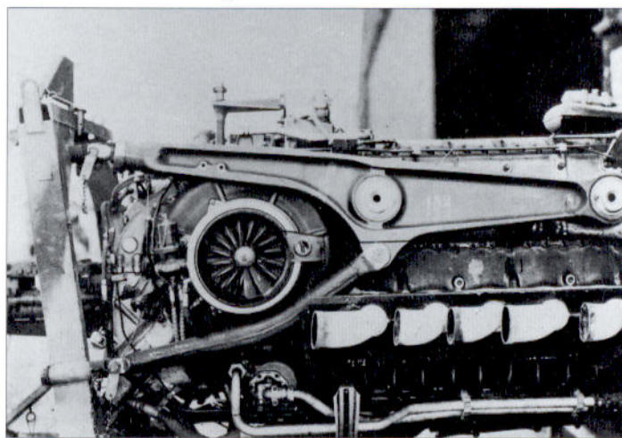
Junkers Jumo 213E with engine-mounted cannon.
