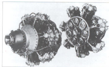
BMW 803 28-cylinder liquid-cooled radial engine.
